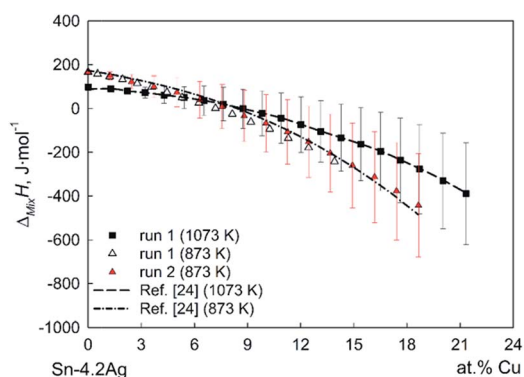
Fig. 1 Integral enthalpy of mixing of liquid (Sn-4.2Ag) 100-x Cu x alloys.
