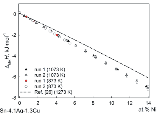
Fig. 2 Integral enthalpy of mixing of liquid (\text{Sn-4.1Ag-1.3Cu})_{100-x}\text{Ni}_x alloys.
