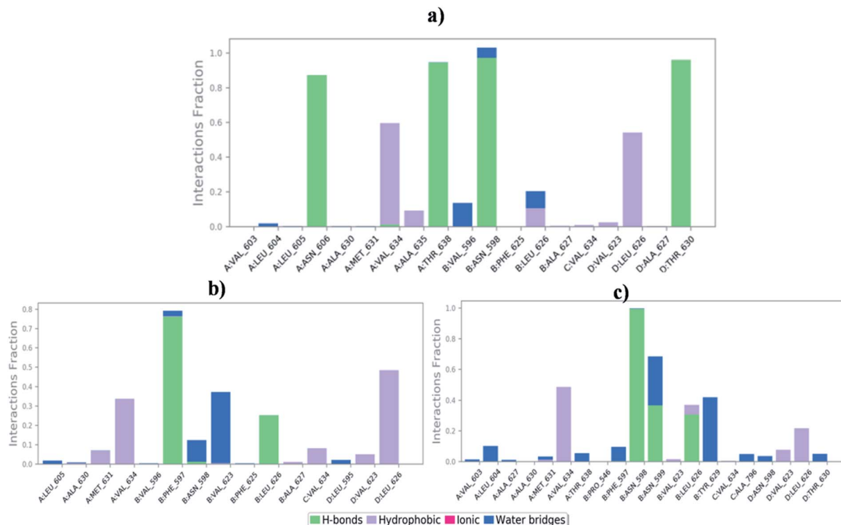
Fig. 7 Bar-chart representation of protein–ligand contacts of (a) NM28 –5UN1 complex, (b) MK-801 –5UN1 complex and (c) Hupa –5UN1 complex during molecular dynamics simulation.
