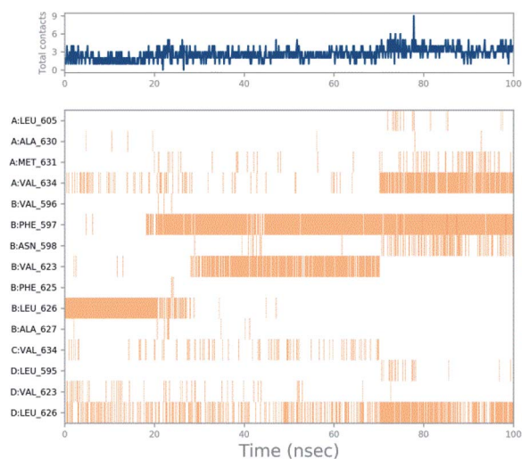
Fig. 9 Timeline representation of ligand–protein contacts for compound MK-801 –5UN1 complex observed during molecular dynamics simulation.
