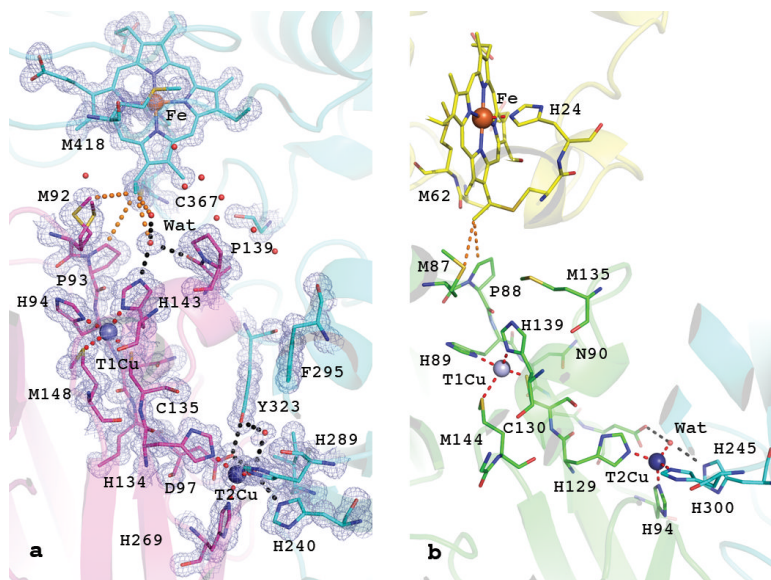
Fig.2. Details of interaction between cytochrome and Cu binding domains for (a) RpnNIR and (b) AxNIR-Cyt 551 complex 6 with shortest distances between heme and Cu binding domain shown as dotted orange lines. An ET route can be traced from the porphyrin CBC atom via a water molecule, the Ne2 atom of the His143 ligand of the T1Cu centre. For RpnNIR -P2 13 monomer-A, 2Fo-Fc map contoured at 1.0 \sigma for the T1Cu and T2Cu Sites for. Fe-T1Cu distance is 10.4Å, T1-T2Cu is 12.7Å. For simplicity only one conserved water molecule on the shortest route to T1Cu is shown at the interface between cytochrome domain and T1Cu. This water is located in very close proximity to both CBC heme atom (3.6Å) and Ne2 atom of Cu ligating His143 (2.8Å). The binary complex, AxNIR-Cyt 551 , has a hydrophobic interface between Cytochrome 551 and T1Cu site.
