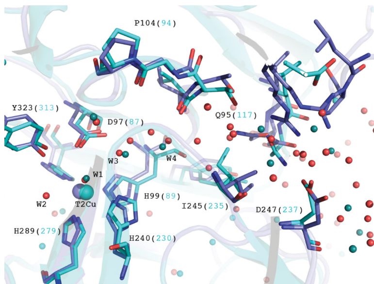
Fig.4. Details of the proton pathway in RpNiR (dark blue with water as red sphere) and its comparison with P/NiR (light blue) (PDB, 2zoo). This channel is comprised of residues on the interface between two monomers that extends from the T2Cu catalytic centre to the protein surface and is filled with an extensive water network. In the case of P/NiR the channel is interrupted by Ile 235 that has a different orientation to the corresponding Ile245 of RpNiR . Ile235/245 in these extended NiRs correspond to conserved His254 residue in two domain AxNiR 23 .
