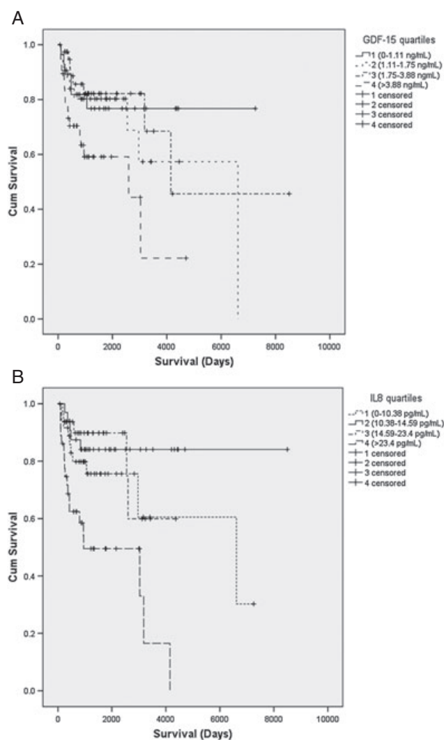
Figure 2 Kaplan–Meier survival curves according to GDF15 quartiles (ng/mL, A) and to IL-8 quartiles (pg/mL, B).
