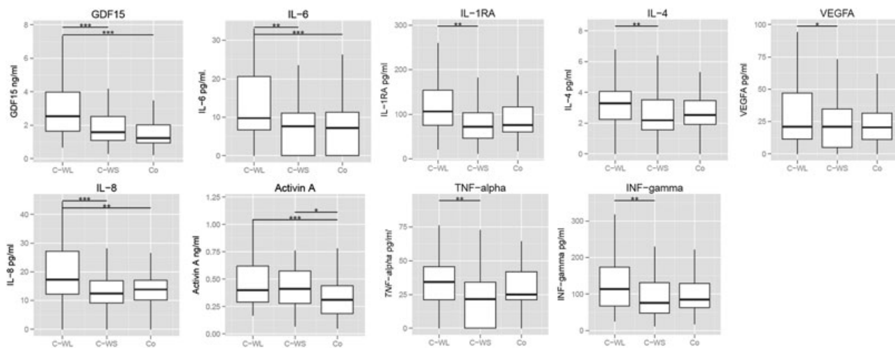
Figure 1 Upregulated cytokine levels in weight losing patients with cancer. Data are represented as box plots (median and quartiles). Circulating levels of cytokines in control patients (Co), weight stable cancer patients (C-WS), and weight losing cancer patients (C-WL). Non-parametric one-way ANOVA Kruskal–Wallis test and multiple comparisons test Dunn's * P < 0.05 , ** P < 0.01 , *** P < 0.001 .
