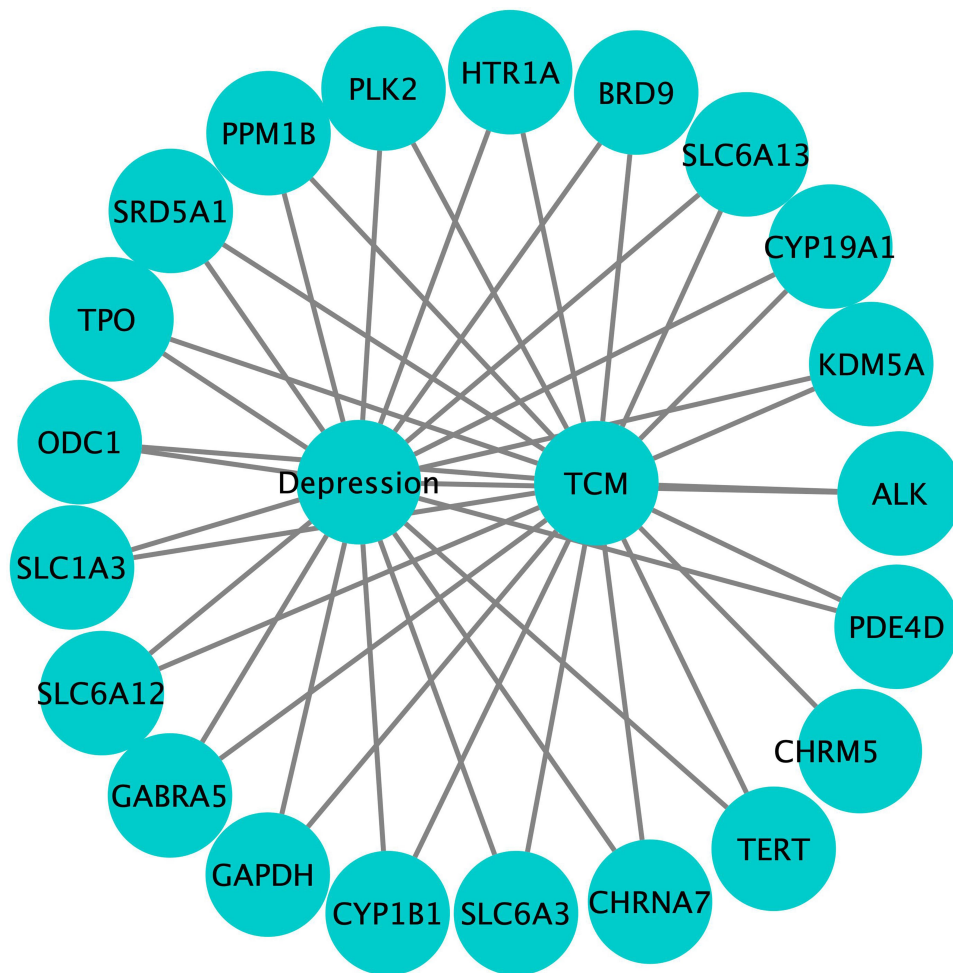
Figure 4 A total of 21 targets were used to establish the regulation network in Cytoscape. Abbreviation: JZG, Jiuwei Zhenxin granules.
