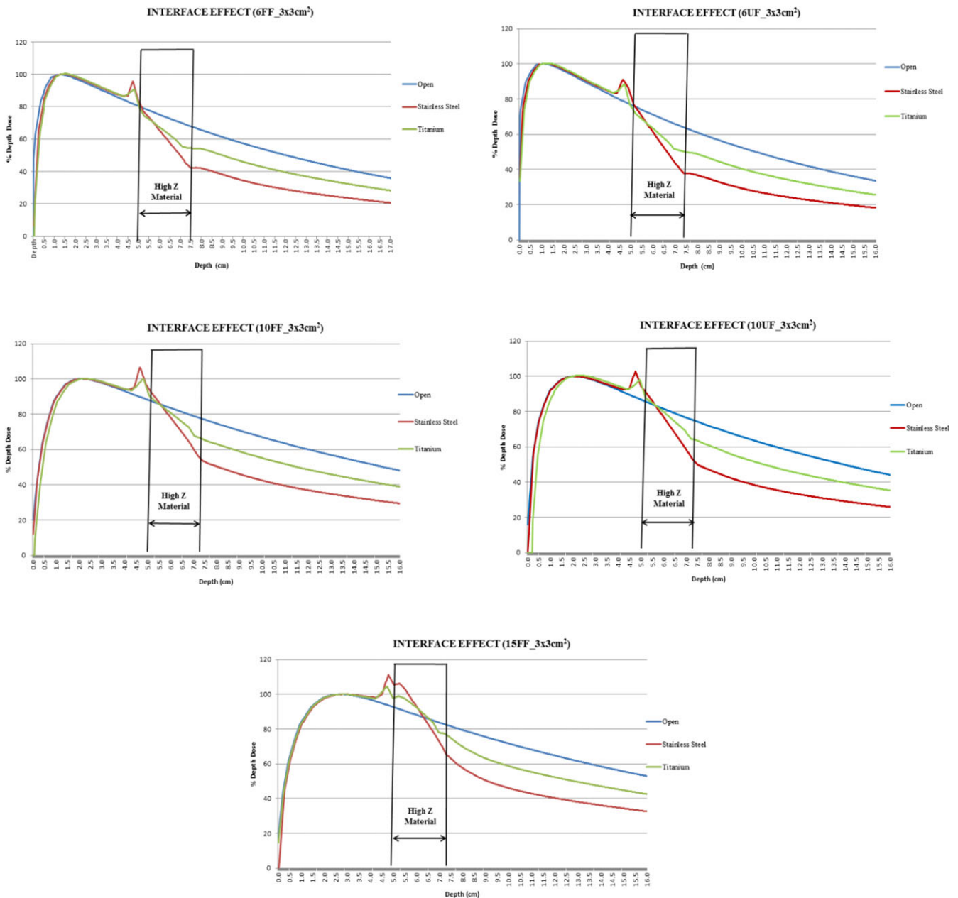
FIG. 2. Interface effect observed at high Z material interfaces in PDD calculated by Acuros XB algorithm (Absorbed Dose to Medium) for field size 3 \times 3 \text{ cm}^2 .
