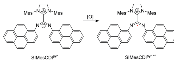
Fig. 15 NHC–CDI distonic radical cation reported by Johnson and co-workers. 45 (Mes = 2,4,6-trimethylphenyl, [O] = oxidant).
