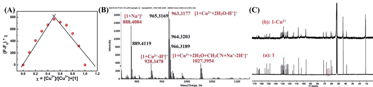
Fig. 7 (A) Job's plot for the complexation of 1 with \text{Cu}^{2+} , indicating the formation of a 1 : 1 complex. The total [\mathbf{1}] + [\text{Cu}^{2+}] = 40 \mu\text{M} . (B) ESI-MS spectrum of 1\text{-Cu}^{2+} . (C) ^{13}\text{C} NMR spectra of 1 upon addition of \text{Cu}^{2+} in \text{CD}_2\text{Cl}_2 .
