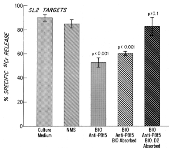
FIG. 2. Ability of B10 anti-P815 serum to inhibit tumor-specific lysis before absorption and after absorption with B10 or B10.D2 lymphocytes. P values are given for each antiserum in comparison to NMS.
