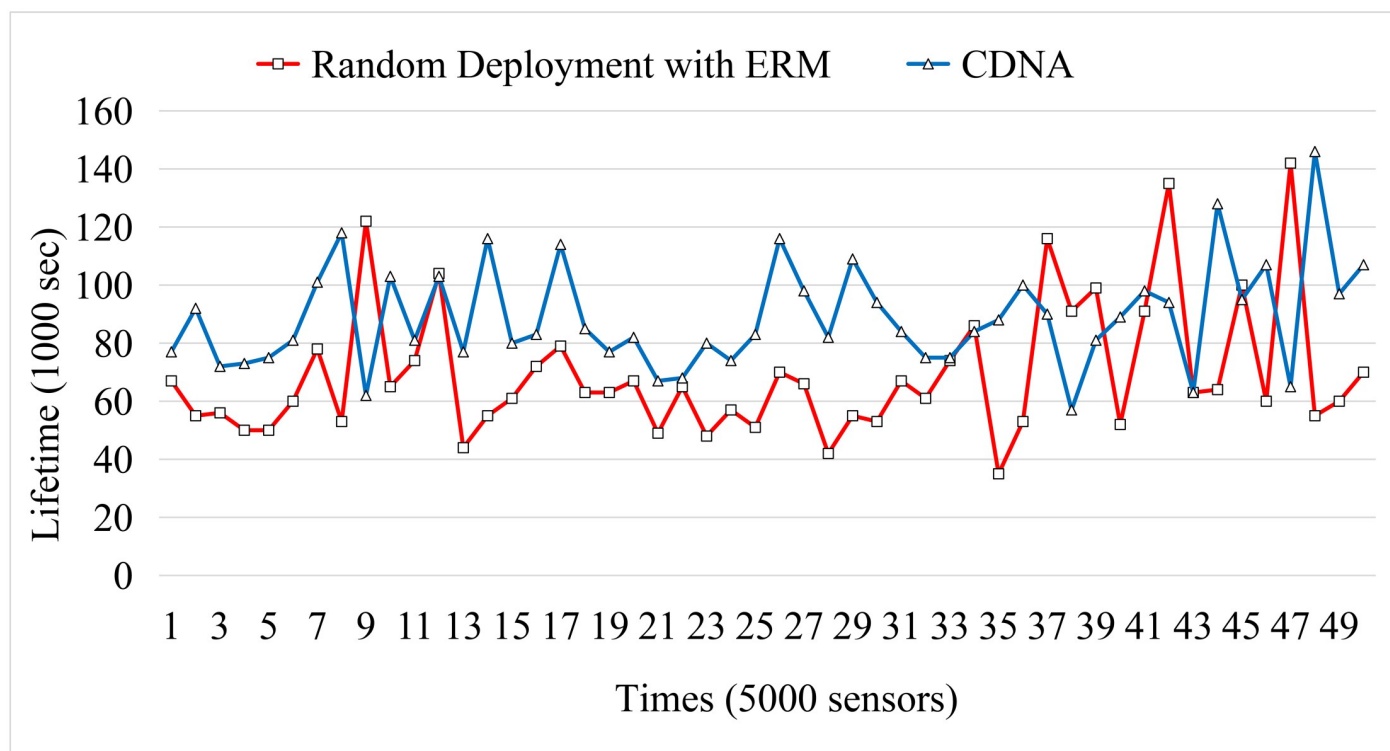
Fig 13. Network lifetime compare for 5000 sensors.
