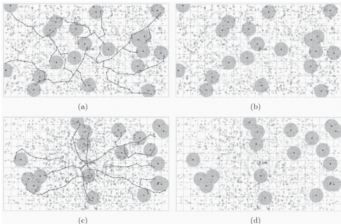
Fig 9. The event monitoring and energy hole problem relieving simulation: (a) The event monitoring and route construction results in the random deployed environment; (b) The network lifetime is over, when the energy hole appears in random deployment environment; (c) The events monitoring in \chi^2 distribution deployment environment; (d) The network lifetime is over, when the energy hole appears in \chi^2 distribution deployment environment.
