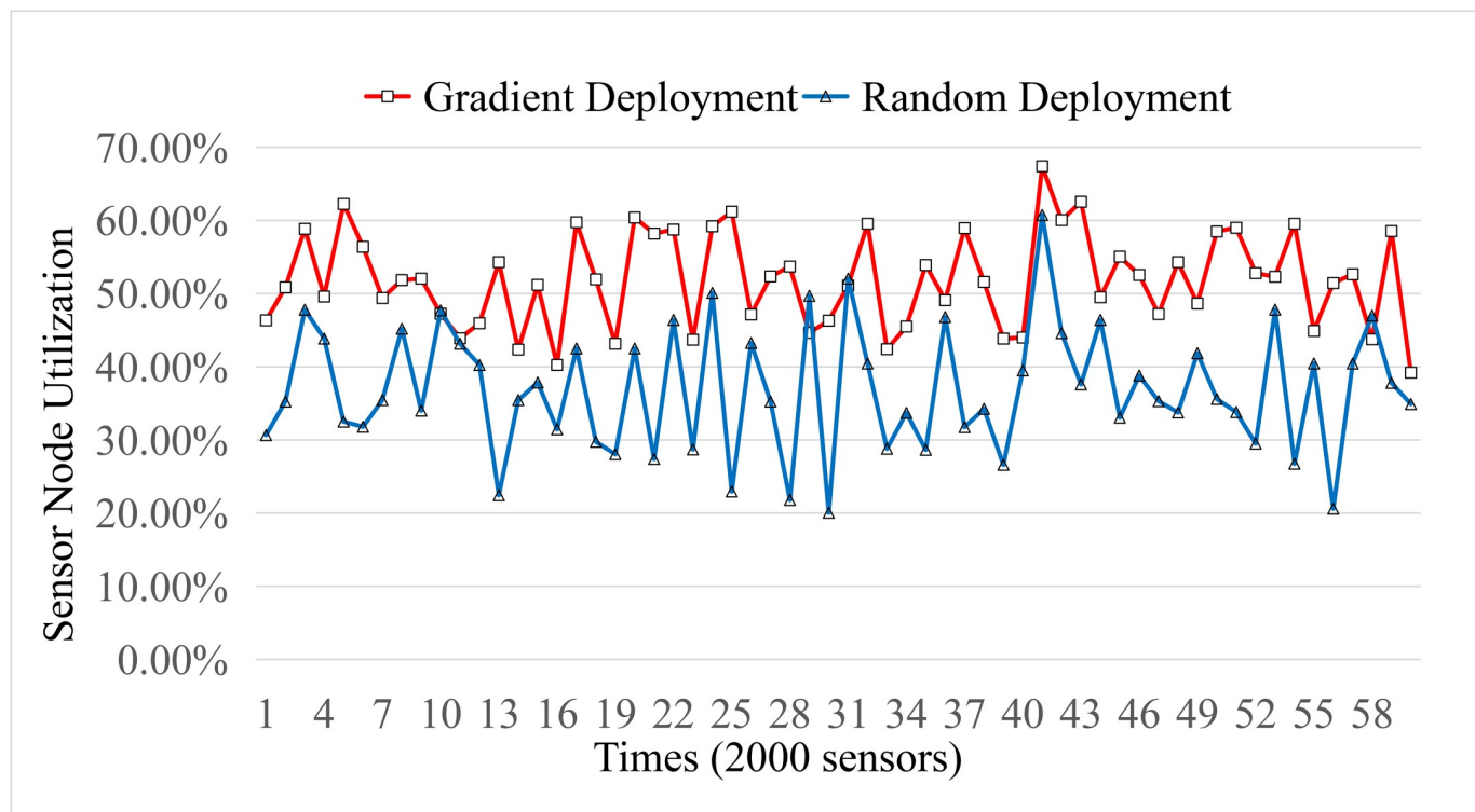
Fig 10. Sensor utilization.
