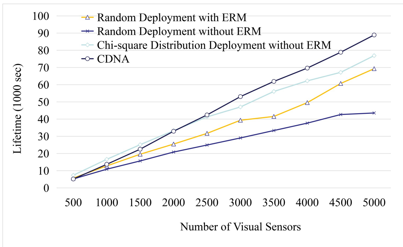
Fig 14. Network lifetime compare.
