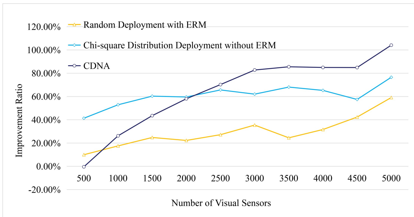
Fig 15. Lifetime comparison.
