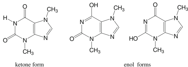
Fig. 2 Tautomeric forms of theobromine
