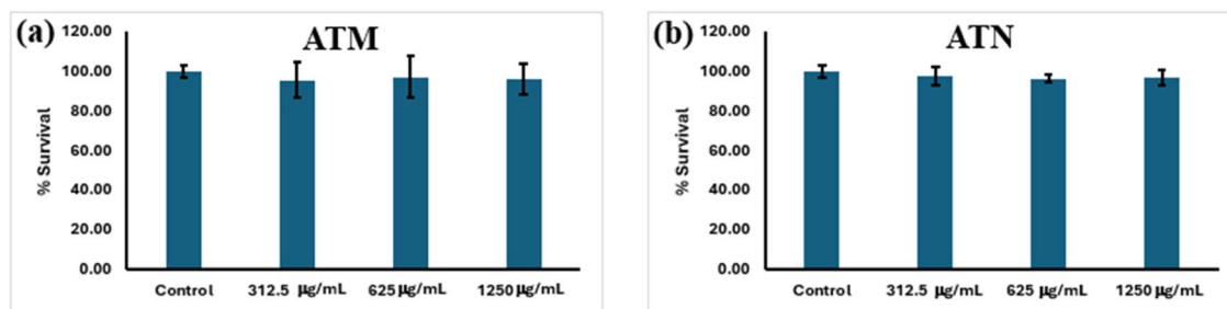
Fig. 7 (a and b) Percent cell viability of rat fibroblast cells treated with ATN and ATM (1/2×, 1×, and 2× of MIC) compared with the vehicle-treated cells using MTT [3-(4,5-dimethylthiazol-2-yl)-diphenyltetrazolium bromide] (mean ± SEM ( n = 4)).
