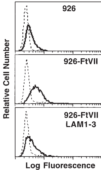
Figure 1. L-selectin binds ligands expressed on (top) 926 and (middle) 926-FtVII cells. Cells were stained in indirect immunofluorescence assays with L'IgM (10 \mu g/ml) and FITC-labeled goat anti-mouse IgM antibody, and analyzed by flow cytometry. (Bottom) 926-FtVII cells were stained with L'IgM (10 \mu g/ml) that was preincubated with a function-blocking anti-L-selectin mAb (LAM1-3, 50 \mu g/ml) for 20 min. The dotted lines represent background staining with an unreactive mouse IgM antibody (HB13b, 10 \mu g/ml), with secondary antibody alone, or with L'IgM in the presence of 5 mM EDTA. Results represent those obtained in three experiments and with two independent lines of 926-FtVII cells.
