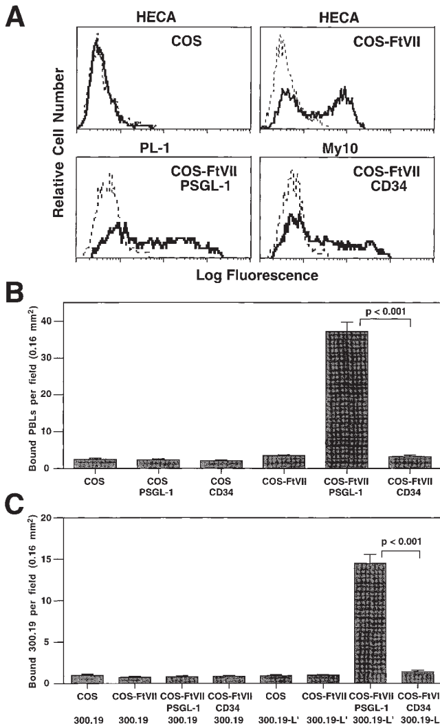
Figure 7. CLA expression alone is insufficient for L-selectin binding. (A) Staining of COS and COS-FtVII cells with the HECA-452 (10 \mu\text{g}/\text{ml} ), PL-1 (anti-PSGL-1, 10 \mu\text{g}/\text{ml} ), and My10 (anti-CD34, 10 \mu\text{g}/\text{ml} ) mAbs in indirect immunofluorescence assays with flow cytometry analysis. Dashed lines represent cell staining with equivalent amounts of unreactive, isotype-matched control antibodies or with secondary antibody alone. (B) Binding of lymphocytes (PBLs) to COS or COS-FtVII cells transiently transfected with cDNAs encoding PSGL-1 or CD34 in a nonstatic binding assay. (C) Binding of 300.19 or 300.19-L' cells to COS or COS-FtVII cells transiently transfected with cDNAs encoding PSGL-1 or CD34 as indicated in a nonstatic binding assay. Values in B and C represent the mean ( \pm SEM) number of lymphocytes bound to COS cells in at least 30 randomly chosen microscopic fields as previously described (8). All results represent those obtained in three independent experiments.
