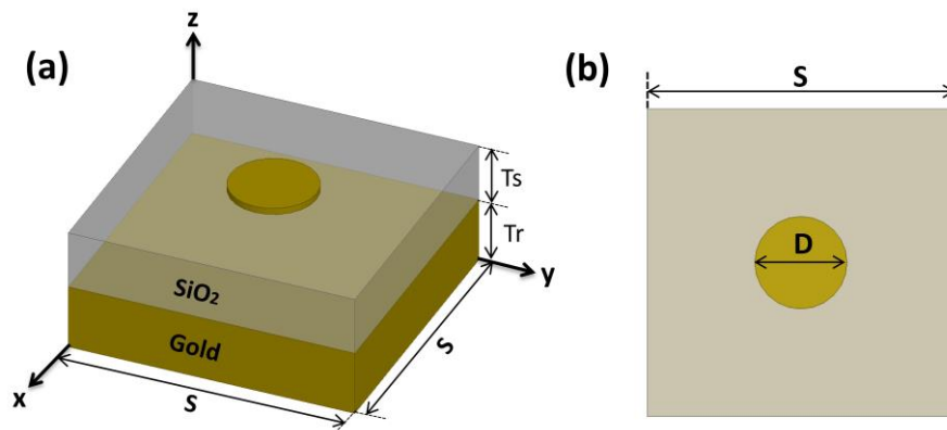
Figure 2. (a) Schematic view of the circular nanodisk mounted on the SiO 2 grounded substrate with T_s and T_r of 40 and 200 nm, respectively. (b) Top view (the x - y plane) with a circular nanodisk diameter ( D ) of 235 nm and a substrate size ( S ) of 1.3 \mu\text{m} .
