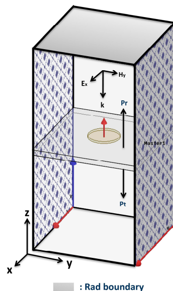
Figure 1. Schematic view of the circular nanodisk array simulation using a periodic boundary condition. Master and slave boundaries are used along the x - z and y - z planes, and the radiation boundaries are assigned on the top and bottom of the simulation boundary box.
