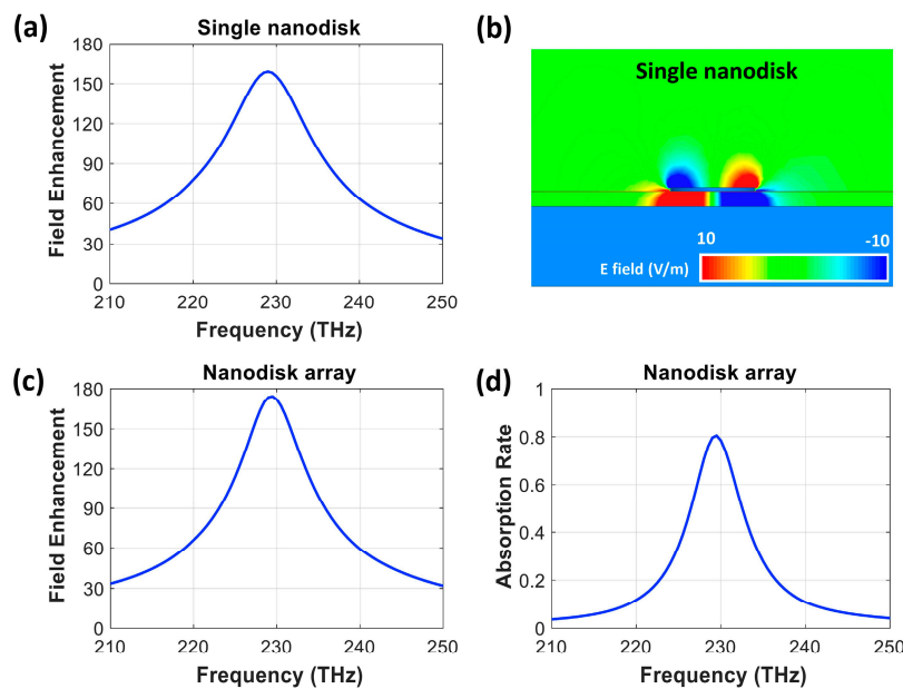
Figure 3. The performance of the single nanodisk and the nanodisk array on the grounded SiO 2 substrate. (a) The electric field enhancement of the single nanodisk with a disk diameter ( D ) of 235 nm and a SiO 2 thickness ( T_s ) of 40 nm. (b) The z component of the electric field distribution ( E_z ) in the x - z plane along the disk's central axis. (c) The electric field enhancement and (d) the absorption rate of the nanodisk array with an antenna pitch size ( P ) of 1 \mu\text{m} .
