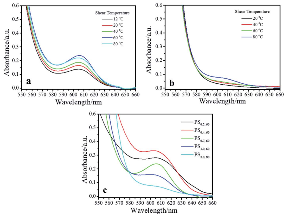
Fig. 4 UV-vis absorption spectra of (a) PS_{0.7} and (b) PS_{5.0} sheared at different temperatures. (c) UV-vis absorption spectra of sheared P3HT solutions with different concentrations. The shear temperature of PS_{5.0} is 80\text{ }^{\circ}\text{C} , and the shear temperature of the other solutions is 60\text{ }^{\circ}\text{C} . The shear rate is 1.0\text{ s}^{-1} .
