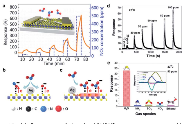
Fig. 15 (a) Response of the Ag NW/WS 2 gas sensors upon NO 2 exposure (25, 50, 100, 200, and 500 ppm). (b) Schematic of the adsorption of NO 2 molecules on the WS 2 surface catalytically enhanced by Ag NWs. (c) Schematic of electron transfer from the Ag NWs and increase of the electron concentration of WS 2 . 94 Adapted with permission from ref. 94. Copyright 2016 American Chemical Society. (d) Response curves toward different concentrations of H 2 S. (e) Selectivity of the optimal gas sensor employing SnO 2 /rGO nanocomposites. Inset: response curves upon exposure to the corresponding analytes. 95 Adapted with permission from ref. 95. Copyright 2016 American Chemical Society.
