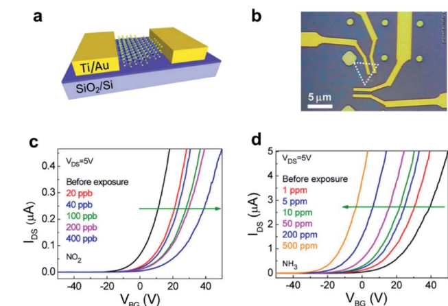
Fig. 2 (a) Schematic illustration of the \text{MoS}_2 FET (back-gate) as a gas sensor. (b) Optical image of two separate devices. (c and d) Transfer characteristics of the \text{MoS}_2 FET upon exposure to \text{NO}_2 and \text{NH}_3 of varied concentrations, respectively. 50 Adapted with permission from ref. 50. Copyright 2014 American Chemical Society.
