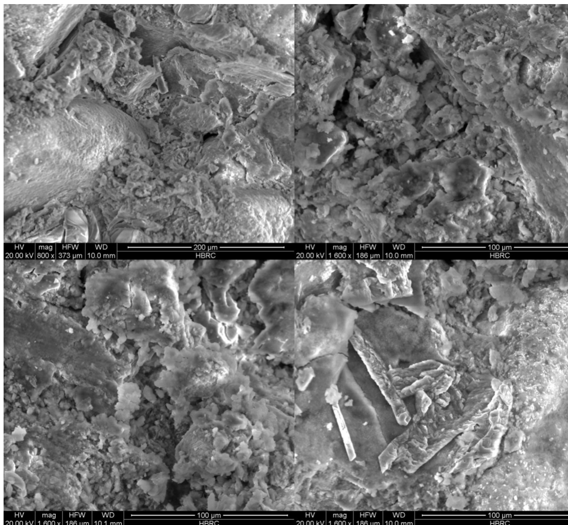
Figure 7 SEM images of cement mortar specimen MNN00 (control).
