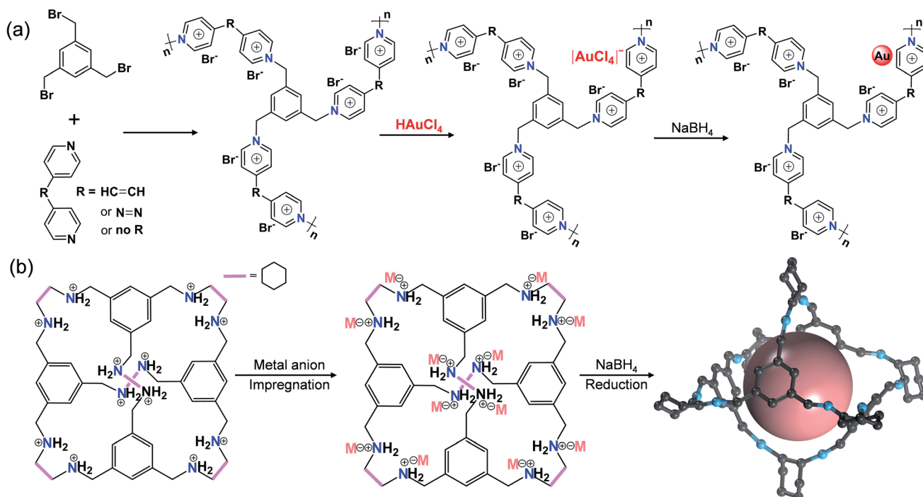
Fig. 11 Cases of POPs or POCs for ion-confinement. Schematic illustration of constructing (a) Au@PION and (b) MCs@I-Cage-Cl.
