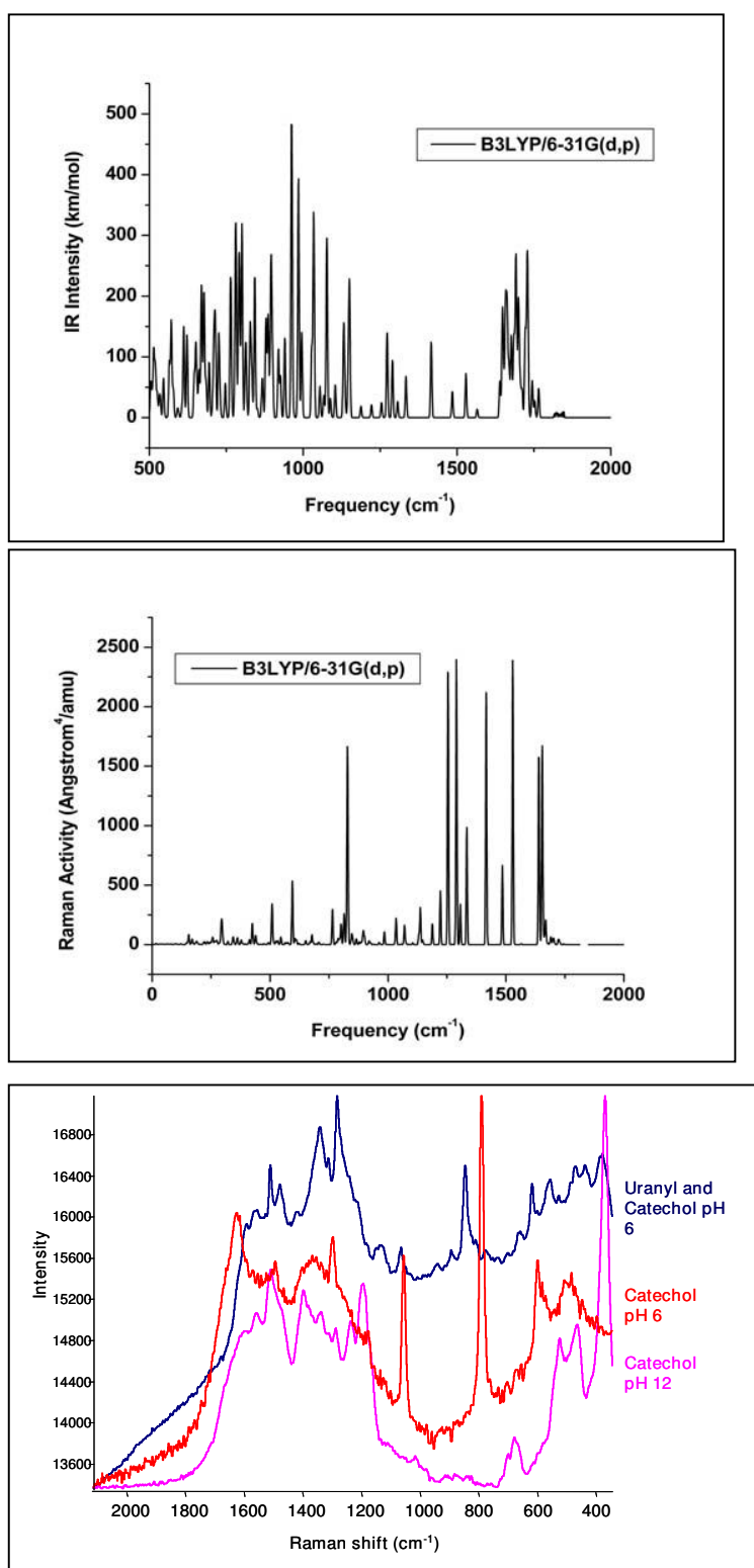
Figure 8 Calculated (a) IR and (b) Raman spectra of \text{UO}_2(\text{OH})_2 \cdot 2\text{H}_2\text{O} results in vibrational frequencies consistent with the (c) observed Raman spectrum of uranyl-catechol solutions at pH 2.
