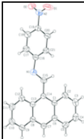
Fig. 1. Molecular structure of the title compound with the atom numbering scheme. Displacement ellipsoids are drawn at the 30% probability level. H atoms are presented as a small cycles of arbitrary radius.
