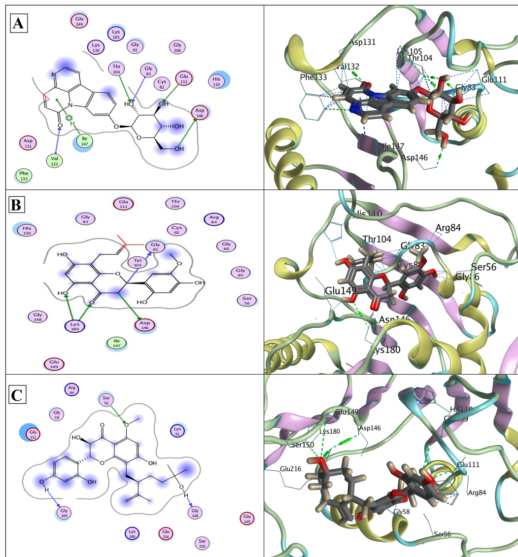
Figure 6. (A) Docked Canthin-6-one 9-O-beta-glucopyranoside in complex with NS5 RNA CAP (PDB ID: 3P97); showing hydrogen bonds to the back-bone of GLY83 and VAL132, and to side chains of THR104, GLU111 and ASP146. An arene interaction with ILE147 is also shown. (B) Docked Kushenol W in complex with NS5 RNA CAP (PDB ID: 3P97); showing hydrogen bonds to the back-bone of GLY81, and to side chains of ASP146 and LYS180. (C) Docked Kushenol K in complex with NS5 RNA CAP (PDB ID: 3P97); showing hydrogen bonds to the side chain of SER56, and back-bone of GLY109 and GLY148. LigX 2D interaction analysis shown at left and 3D interaction analysis shown at right side.
