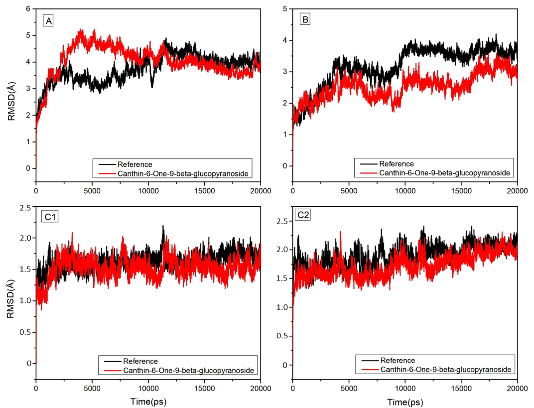
Figure 9. RMSD of Canthin-6-One 9-O-Beta-Glucopyranoside complexed to NS1 (A), NS3/N2B Chimera (B), NS5 RNA Pocket (C1) and SAM pocket (C2) with respect to their unbound (apo) reference structures.
