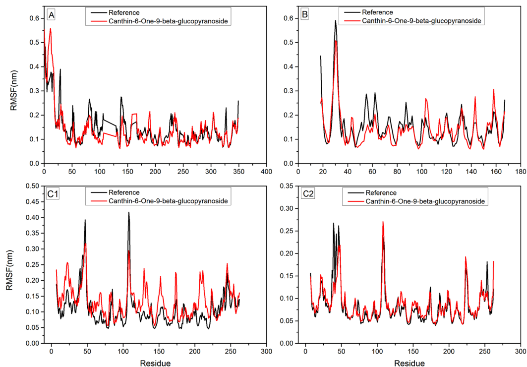
Figure 10. Root mean square fluctuations (RMSF) of Apo ((A) NS1 (B) NS3 (C1) NS5/RNA and (C2) NS5/SAM compared to complexed states for 20 ns Simulation, Respectively.
