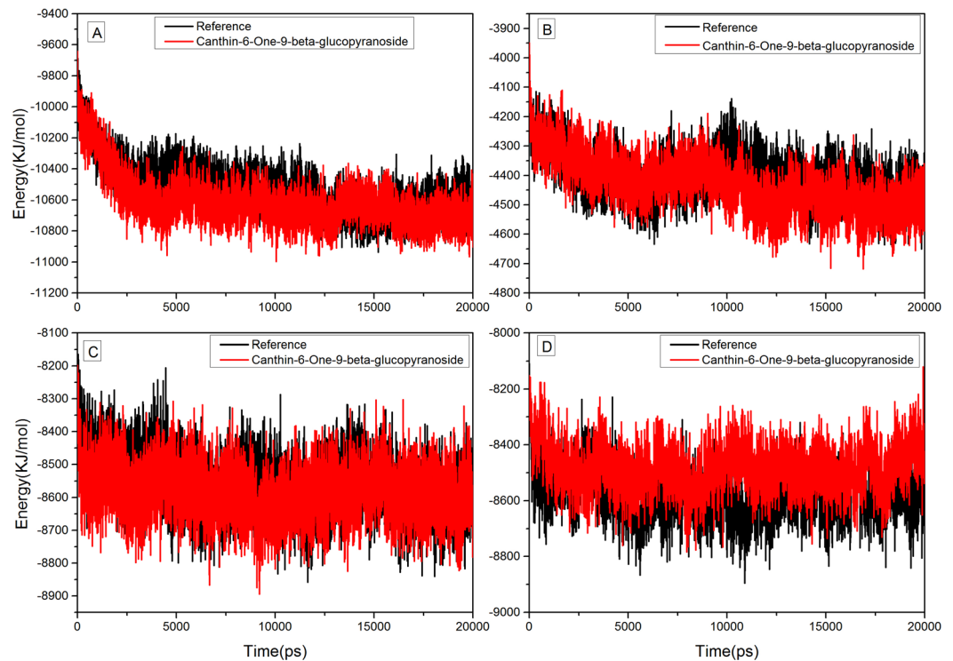
Figure 8. MD trajectories for NS1, NS3, NS5-RNA and NS5-SAM bound with and without Canthin-6-one 9-O-beta-glucopyranoside superposed over each other.
