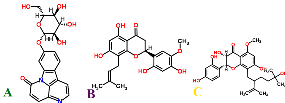
Figure 3. 2D chemical structures of three top ranked multiple DV serotypes inhibitors. (A) Canthin-6-one 9-O-beta-glucopyranoside, (B) Kushenol W and (C): Kushenol K.
