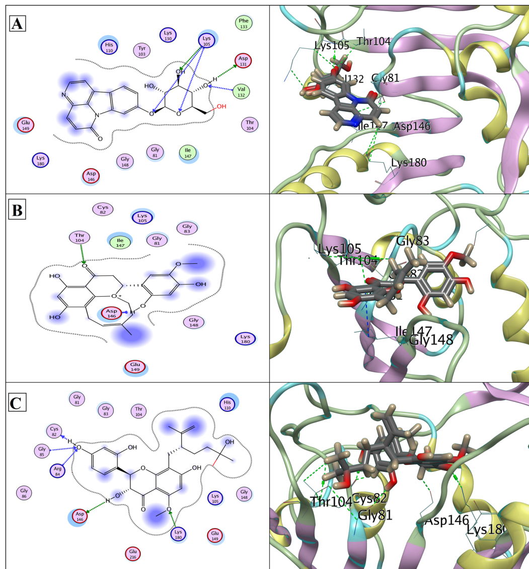
Figure 7. (A) Docked Canthin-6-one 9-O-beta-glucopyranoside in complex with NS5 SAM pocket (PDB ID: 3P97); showing hydrogen bonds to the side chain/back-bone of LYS105, to the side chain of ASP131, and to the back-bone of VAL132. (B) Docked Kushenol W in complex with NS5 SAM pocket (PDB ID: 3P97); showing hydrogen bonds to the side chain of THR104, and to the back-bone of ASP146. (C) Docked Kushenol K in complex with NS5 SAM pocket (PDB ID: 3P97); showing hydrogen bonds to back-bones of CYS82, GLY85 and ARG84, and to side chains of ASP146 and LYS180. LigX 2D interaction analysis shown at left and 3D interaction analysis shown at right side.
