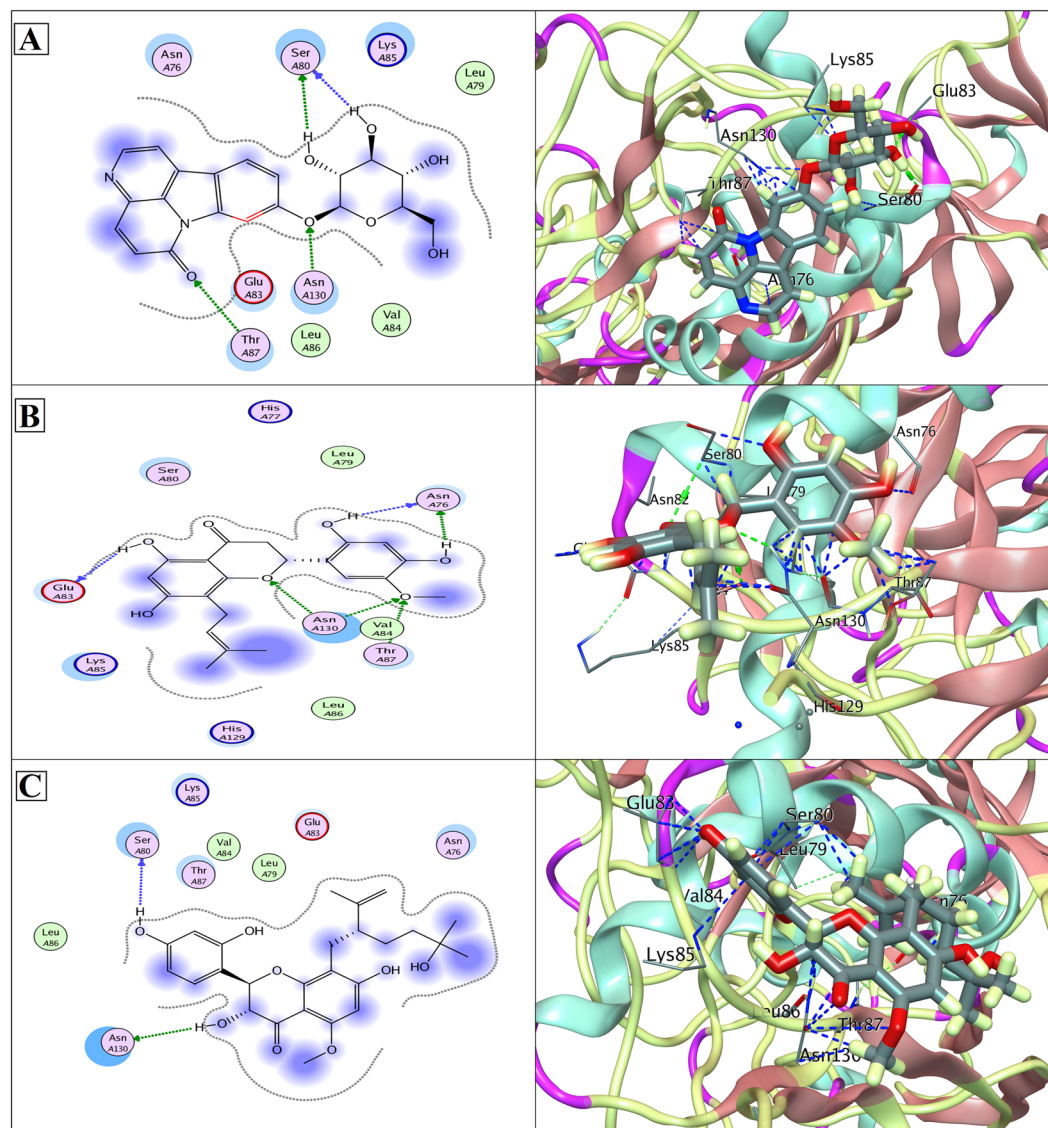
Figure 4. (A) Docked Canthin-6-one 9-O-beta-glucopyranoside in complex with NS1 protease (PDB ID: 4O6B); showing hydrogen bonds with the side chain/back-bone of SER80, and to side chains of THR87 and ASN130. (B) Docked Kushenol W in complex with NS1 protease; showing hydrogen bonds to the side chain/back-bone of ASN76, to the back-bone of GLU83, and to side chains of THR87 and ASN130. (C) Docked Kushenol K in complex with NS1 protease (PDB ID: 4O6B); showing hydrogen bonds to the back-bone of SER80 and to the side chain of ASN130. LigX 2D interaction analysis shown at left and 3D interaction analysis shown at right side.
