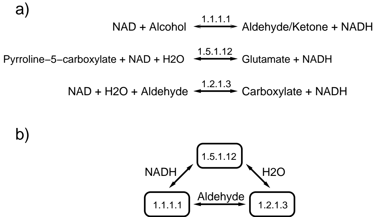
Figure 4 Minimal path length (MPL) between enzymes. a) The reactions catalyzed by EC 1.1.1.1 (alcohol dehydrogenase), EC 1.5.1.12 (l-pyrroline-5-carboxylate dehydrogenase) and EC 1.2.1.3 (aldehyde dehydrogenase). b) There are several paths leading from EC 1.1.1.1 to EC 1.2.1.3. The shortest path goes from EC 1.1.1.1 through aldehyde to EC 1.2.1.3 and is of length 1 (MPL = 1).
