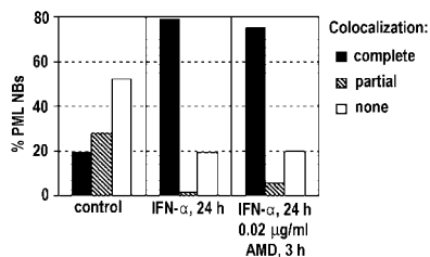
Figure 5. Quantification of the colocalization of PML NBs and NDH II in control cells, in IFN- \alpha -stimulated cells, and after inhibition of POL I transcription ( 0.02 \mu\text{g/ml} AMD; 3 h) performed in confocal images described in Fig. 2 ( n = 20 ). Because there is no colocalization after inhibition of POL II transcription ( 100 \mu\text{g/ml} \alpha -amanitin for 3 h; Fig. 2, C and D) the quantification was not performed in this case. In control cells, NDH II colocalizes completely with 19\% of PML NBs, 28\% of PML NBs colocalize partially, and \sim 53\% do not colocalize with NDH II foci. In IFN- \alpha -treated cells, NDH II colocalizes with 79\% of PML NBs, \sim 2\% colocalize partially, and 19\% of PML NBs do not colocalize with NDH II. After inhibition of POL I transcription, NDH II remains in the association with PML NBs and colocalizes with >75\% of nuclear dots. Less than 5\% of PML NBs colocalize partially, and 20\% do not colocalize with NDH II.
