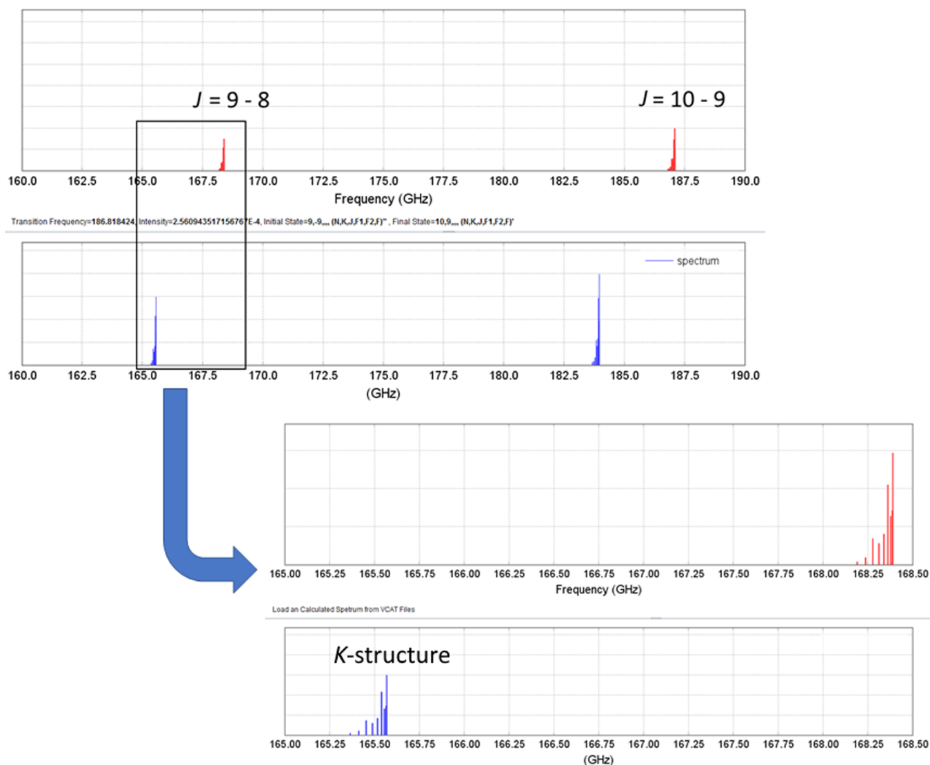
Figure 7. Pure rotational spectrum of CH 3 CN in the 160–190 GHz frequency range: the J = 9 - 8 and J = 10 - 9 rotational transitions. The theoretical spectrum (in red, top panel) has been synthesized by using the equilibrium rotational constants from ref 82 corrected for vibrational contributions at the B2PLYP/m-aug-cc-pVTZ- d H level. A magnified view of the 165–168.50 interval shows the close correspondence between the quantum chemical predictions and the experimental features (in blue, bottom panel).
