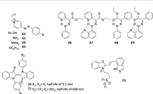
Fig. 14 Overview of the photoresponsive molecules to be discussed for engineering the half-life.
