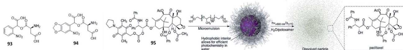
Fig. 16 Overview of discussed PPGs for the stability in water and in the cellular environment. For compound 95, the accompanying figure is reproduced from ref. 87 with permission from The Royal Society of Chemistry, Copyright 2016.
