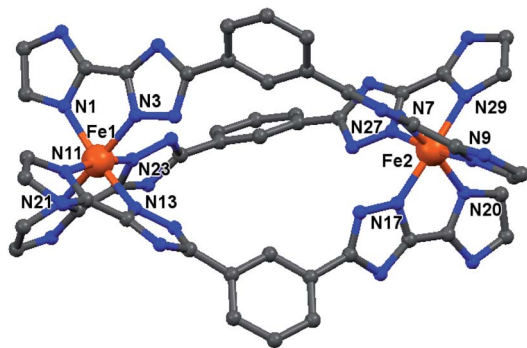
Fig. 3 Molecular structure of the cation of the triply bridged dinuclear helicate, [\text{Fe}_2\text{L}^{2\text{NHIm-meta}}_3]\cdot 2\text{CH}_3\text{CN}\cdot\text{solvent} (1·solvents). The other four helicates are isostructural with this one (see Fig. S7, ESI†). For clarity, the hydrogen atoms, counter-anions and iso-butyl groups are not shown. Colours: Fe orange; N blue; C grey.
