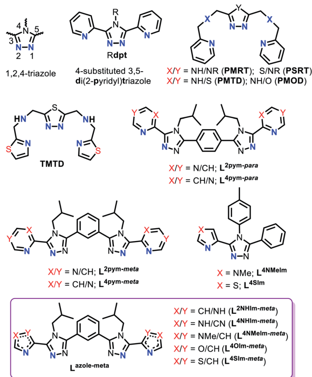
Fig. 2 Generic 1,2,4-triazole numbering (top left), Rdpt ligand (top middle), bis-terdentate PMRT/PSRT/PMTD/PMOD/TMTD (top right and second row left), bis-bidentate azine-triazole Rat ligands ( \text{L}^{2/4\text{pym-meta/para}} ), bidentate azole-triazole Rat ligand ( \text{L}^{4\text{NMe/5Im}} ) and bis-bidentate azole-triazole Rat ligands used in this work (bottom; violet box).
