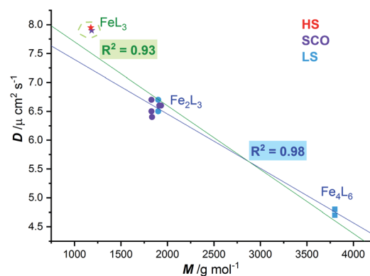
Fig. 5 Correlation (dark blue line, R^2 = 0.98 ) of diffusion coefficient ( D ) with molecular weight ( M ) observed at 298 K for LS Fe 2 L 3 helicites (blue circles) and Fe 4 L 6 cages (blue squares), 57 and the SCO-active Fe 2 L 3 helicites reported here (violet circles). When the two mononuclear Fe II L 3 complexes, one HS and one SCO, are included in the fit, the R^2 only drops to 0.93 (green line), despite them not being members of the Fe 2n L 3n family.
