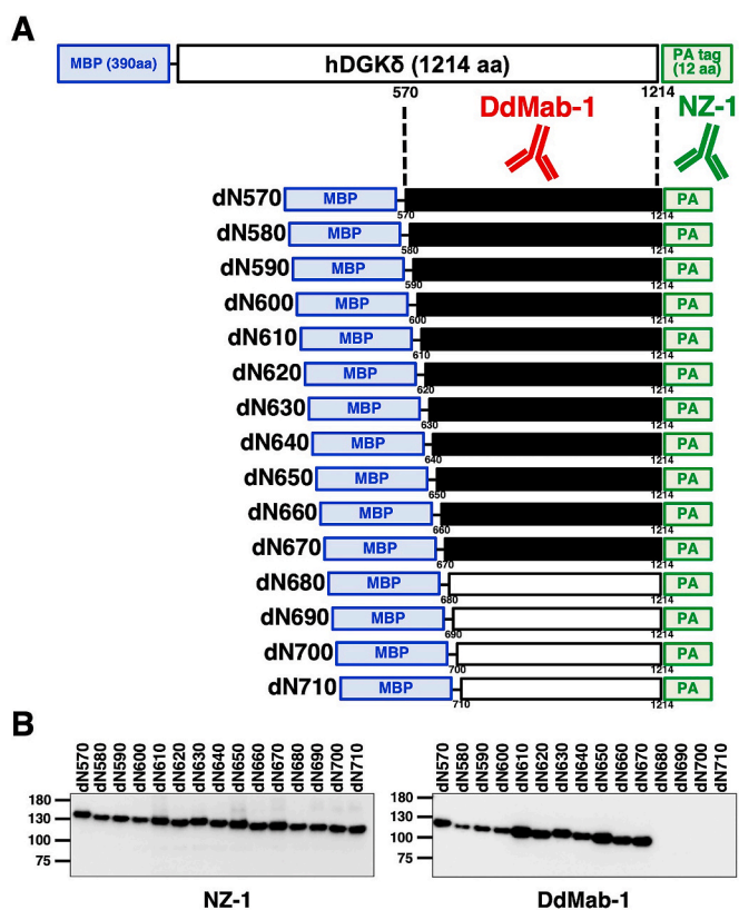
Fig. 1. Epitope mapping of DdMab-1 using deletion mutants of hDGK \delta . (A) Schematic illustration of DdMab-1 epitope mapping. Black bars, deletion mutants detected by DdMab-1. hDGK \delta , human DGK \delta ; MBP, maltose-binding protein. (B) Cell lysates of hDGK \delta N-terminal deletion mutants were electrophoresed, and then transferred onto a PVDF membrane. After blocking, the membrane was incubated with 1 \mu g/ml of DdMab-1 or anti-PA tag antibody (NZ-1).
