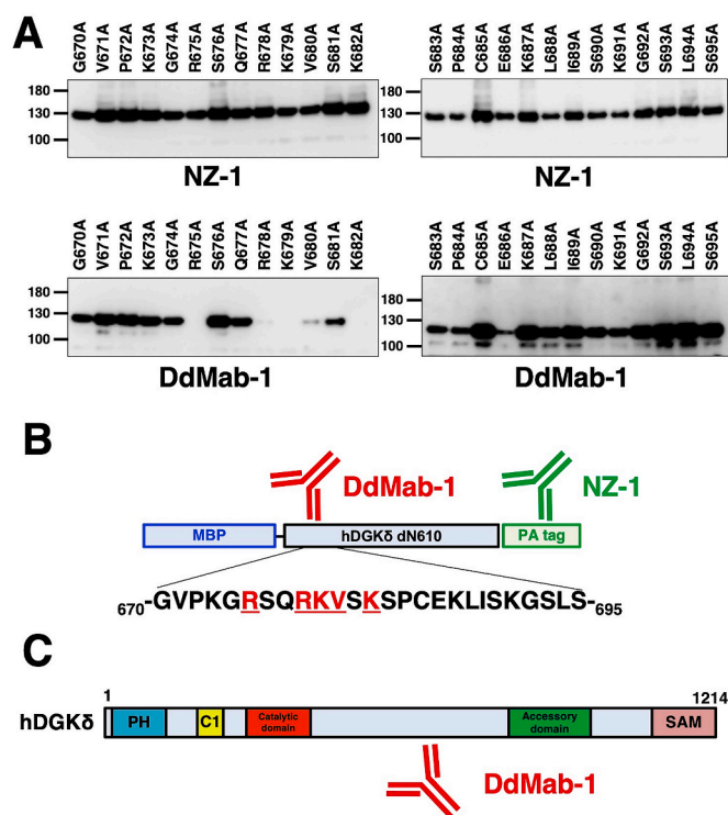
Fig. 2. Epitope mapping of DdMab-1 using point mutants of hDGK \delta . (A) Cell lysates of point mutants of dN610 were electrophoresed, and then transferred onto PVDF membranes. After blocking, the membranes were incubated with 10 \mu g/ml of DdMab-1 or 1 \mu g/ml of anti-PA tag antibody (NZ-1). (B) Schematic illustration of DdMab-1 epitope mapping. Underlined amino acids (Arg675, Arg678, Lys679, Val680 and Lys682) are important for binding of DdMab-1 to hDGK \delta . (C) Schematic illustration of the hDGK \delta structure. DdMab-1 epitope is located in between catalytic and accessory domains. PH, pleckstrin homology; SAM, sterile alpha motif.
