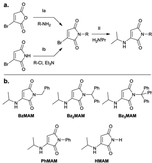
Fig. 1 (a) Synthetic routes for the dye series. To generate the monobromomaleimide (MBM) intermediates, route Ia was followed for all structures except Bz 3 MBM , when it was necessary to adopt route Ib. (b) Structures of the series of dyes used in this work.
