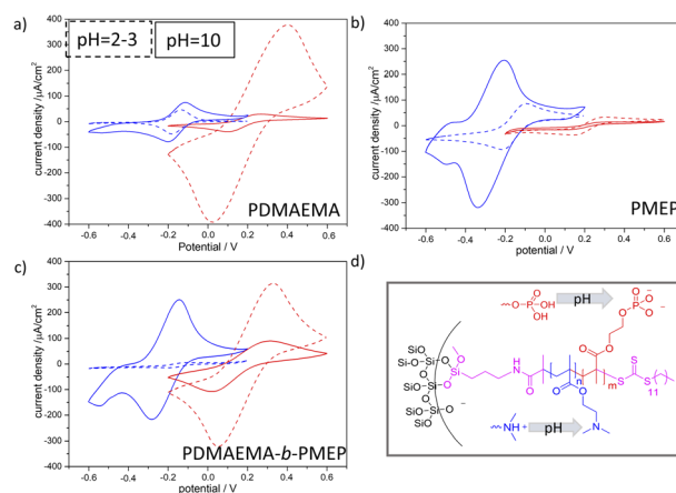
Fig. 4 CV measurements (100 mV s -1 ) of (a) PDMAEMA functionalized (2 h irradiation), (b) PMEPE functionalized (2 h irradiation), (c) PDMAEMA- b -PMEP functionalized mesoporous silicafilm using 0.06 vol% of ethanol. blue) [Ru(NH 3 ) 6 ] 2+/3+ as probe molecule; red) [Fe(CN) 6 ] 3-/4- as probe molecule at concentration of 1 mM in 100 mM KCl electrolyte solution. (d) Schematic illustration of the porous silicafilm in dependence of the pH-value. Cyclic voltammery measurements of PDMAEMA- b -PMEP functionalized mesoporous films were performed on four sets of independently synthesized mesoporous silicafilms.
