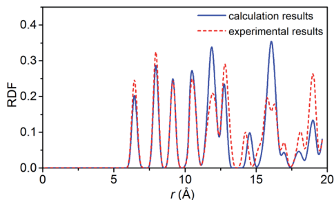
Fig. 2 Comparison of the RDF from ReaxFF-1g (300 K, 0 atm) and from experiment for NONA.
