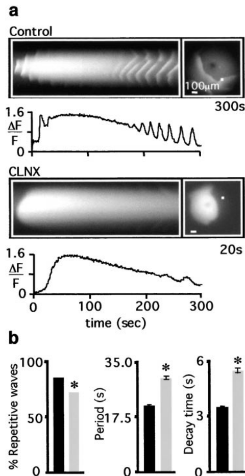
Figure 2. Overexpression of CLNX in Xenopus oocytes inhibits repetitive \text{Ca}^{2+} waves induced by mitochondrial energization. (a) Confocal \text{Ca}^{2+} imaging of a control oocyte ( \text{IP}_3 \sim 300 nM final) energized previously with pyruvate malate (10 mM final). In this representative oocyte, a \text{Ca}^{2+} tide is followed by low-frequency \text{Ca}^{2+} oscillations. \text{Ca}^{2+} oscillations are inhibited in a representative oocyte overexpressing CLNX. Bar, 100 \mu\text{m} . (b) The percentage of oocytes exhibiting repetitive \text{Ca}^{2+} wave activity was decreased in oocytes overexpressing CLNX ( n = 18 , 71%), relative to control oocytes ( n = 25 , 84%) (left). The asterisk indicates statistical significance in comparison to oocytes overexpressing SERCA2b alone, P < 0.05 (Chi-square test). Detailed analysis of \text{Ca}^{2+} waves was performed only on those oocytes that exhibited repetitive \text{Ca}^{2+} activity. Compared with control oocytes, overexpression of CLNX increased the period between waves (middle) and the decay time of individual waves (right). The asterisk denotes a statistical significant difference P < 0.05 ( t test) in comparison to control oocytes (see also Table II).
