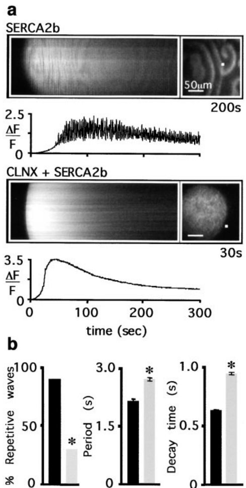
Figure 1. Overexpression of CLNX in Xenopus oocytes inhibits repetitive \text{Ca}^{2+} waves. (a) Confocal \text{Ca}^{2+} imaging in a control oocyte overexpressing rat SERCA2b shows high frequency \text{Ca}^{2+} oscillations after an injection of \text{IP}_3 ( \sim 300 nM final). Inhibition of \text{Ca}^{2+} oscillations is also shown for a representative oocyte coexpressing CLNX + SERCA2b. In this and subsequent figures, the top image contains a spatio-temporal stack of \text{Ca}^{2+} wave activity followed to the right by a representative confocal image of \text{Ca}^{2+} wave activity at the indicated timepoint. Bar, 50 \mu\text{m} . Also in this and subsequent figures, the trace under each image represents the change in fluorescence from resting levels ( \Delta\text{F}/\text{F} ) shown as a function of time. The white square represents the 5 \times 5 pixel area used in determining \Delta\text{F}/\text{F} . (b) The percentage of oocytes exhibiting repetitive \text{Ca}^{2+} wave activity was decreased in oocytes coexpressing CLNX + SERCA2b ( n = 63 , 30%), relative to oocytes overexpressing SERCA 2b alone ( n = 52 , 88%) (left). The asterisk indicates statistical significance in comparison to oocytes overexpressing SERCA2b alone, P < 0.005 (Chi-square test). In this figure and subsequent histograms, the color convention used is as follows: black for SERCA 2b and light gray for CLNX + SERCA2b overexpressing oocytes. Detailed analysis of \text{Ca}^{2+} waves was performed only on those oocytes that exhibited repetitive \text{Ca}^{2+} waves. Compared with oocytes overexpressing SERCA 2b alone, overexpression of CLNX + SERCA2b increased the period between waves (middle) and the decay time of individual waves (right). The asterisk denotes a statistical significant difference P < 0.05 ( t test) in comparison to control oocytes overexpressing SERCA2b alone (see also Table I).
