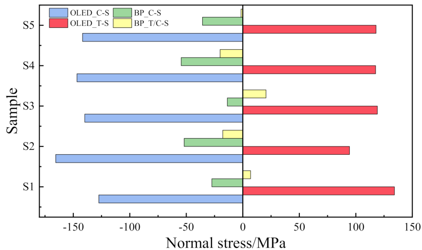
Figure 9. Contrast of normal stress in bending of the central axis with different thickness shapes.
