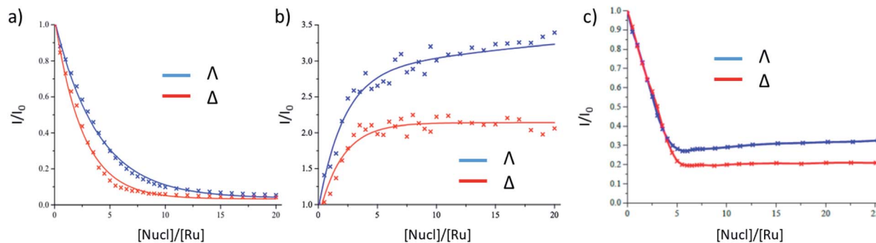
Fig. 2 Steady-state emission titrations of \Lambda/\Delta -[Ru(TAP) 2 (dppz)] 2+ in the presence of (a) poly(dG-dC) (b) poly(dA-dT) (c) salmon-testes DNA. \lambda_{\text{exc}} = 435 \text{ nm} ; \lambda_{\text{em}} = 635 \text{ nm} in 10 mM sodium phosphate buffer in H 2 O. For (a) plots are fitted to the McGhee–von Hippel equation. For (b) and (c) they are best fits using trend-line or interpolation methods. [Ru] = 20 \mu\text{M} (a), 8 \mu\text{M} (b and c).
