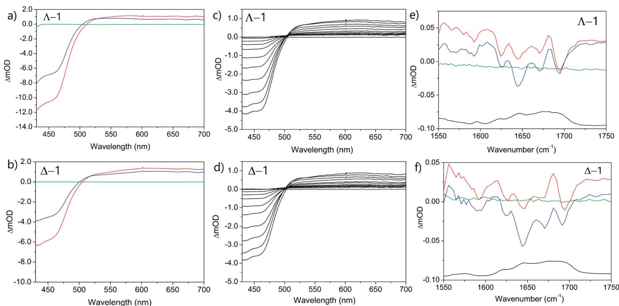
Fig. 7 Transient spectra of \Lambda/\Delta -[Ru(TAP) 2 (dppz)] 2+ in the presence of st-DNA (a and b) ps-TrA spectra at -100\text{ ps} (green), 20\text{ ps} (red), 2500\text{ ps} (blue); (c and d) ns-TrA spectra at selected delays 2 – 5000\text{ ns} ; (e and f) ps-TRIR spectra at -100\text{ ps} (green), 20\text{ ps} (red), 2500\text{ ps} (blue), FTIR (black); \lambda_{\text{exc}} (ps-TrA/TRIR) = 400\text{ nm} , (ns-TrA) = 355\text{ nm} . Pump energy = 1\text{ }\mu\text{J} . In 50\text{ mM} phosphate-buffered \text{D}_2\text{O} pH 7; Nucl/Ru = 25.
