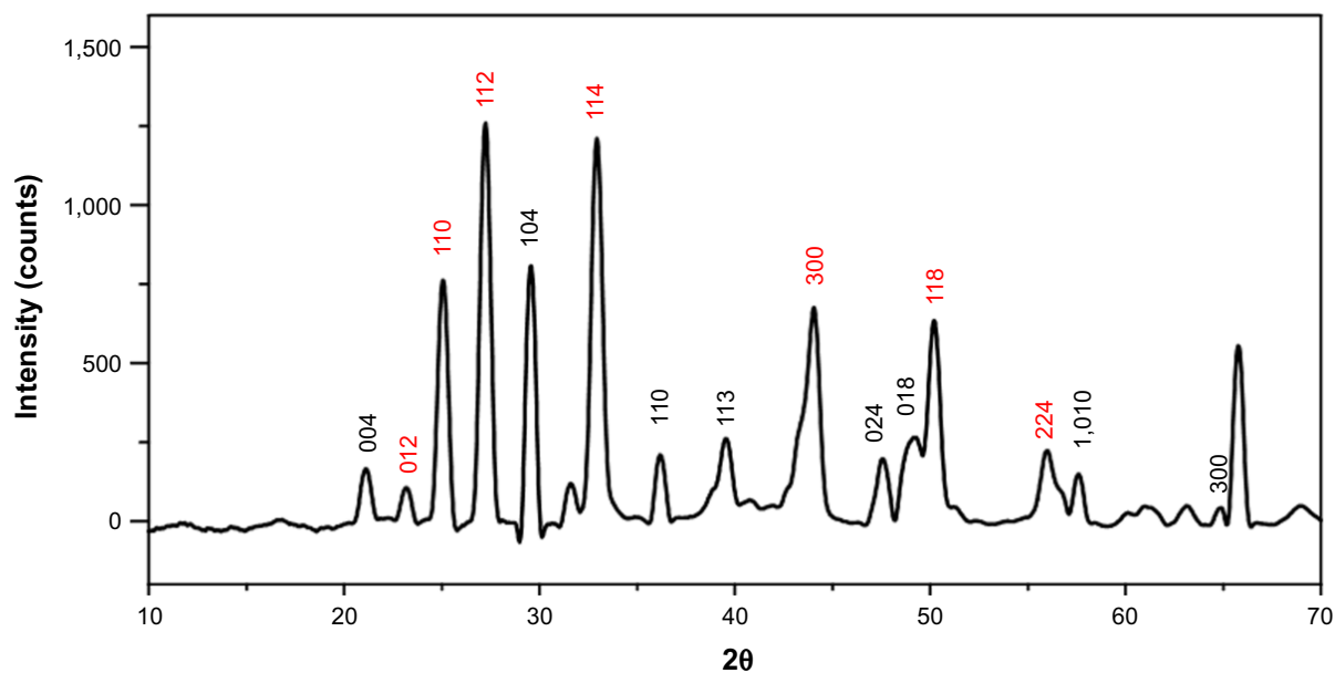
Figure 3 XRD reflections.
