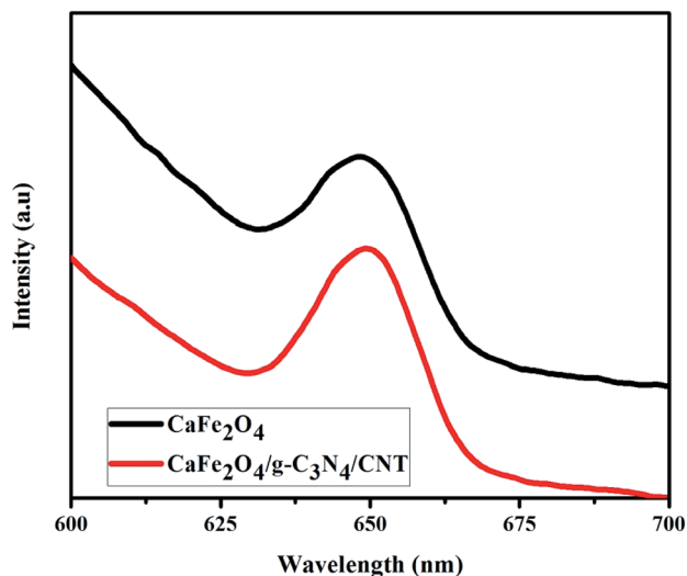
Fig. 8 PL analysis of \text{CaFe}_2\text{O}_4 and \text{CaFe}_2\text{O}_4/\text{g-C}_3\text{N}_4/\text{CNTs} composite.
