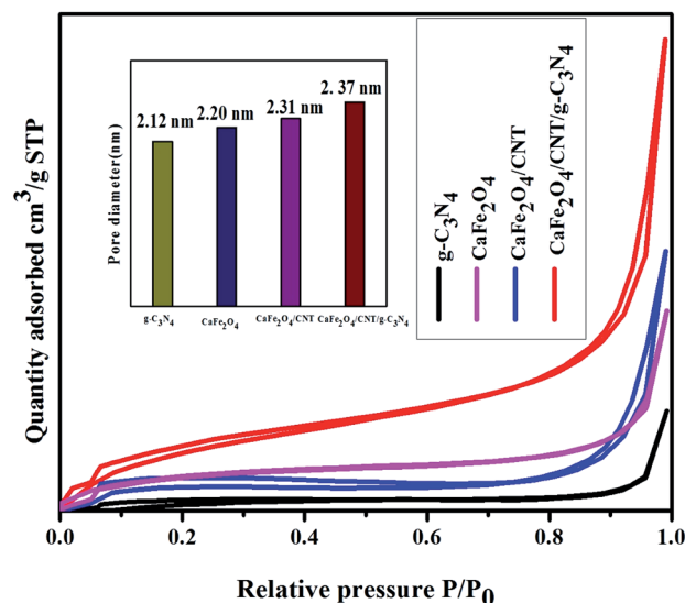
Fig. 9 BET analysis of \text{CaFe}_2\text{O}_4 , \text{g-C}_3\text{N}_4 , \text{CaFe}_2\text{O}_4/\text{CNTs} , and \text{CaFe}_2\text{O}_4/\text{g-C}_3\text{N}_4/\text{CNT} composite.
