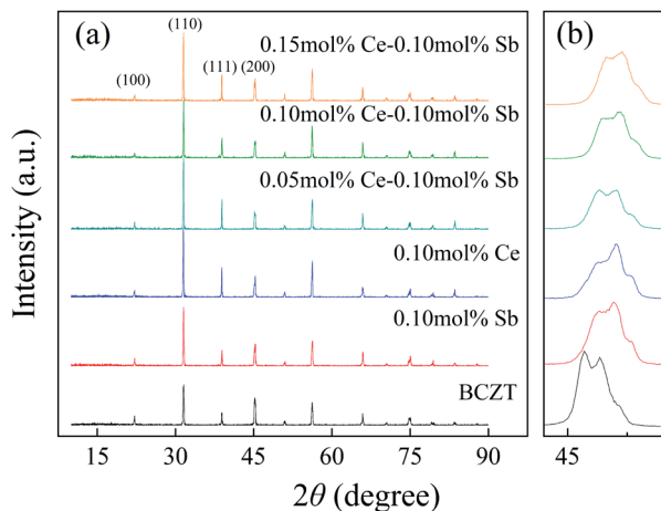
Fig. 1 (a) XRD patterns of BCZTC ceramics prepared by co-doping with Ce and Sb and (b) enlarge patterns near 45^\circ . All the measurements were conducted at room temperature.
