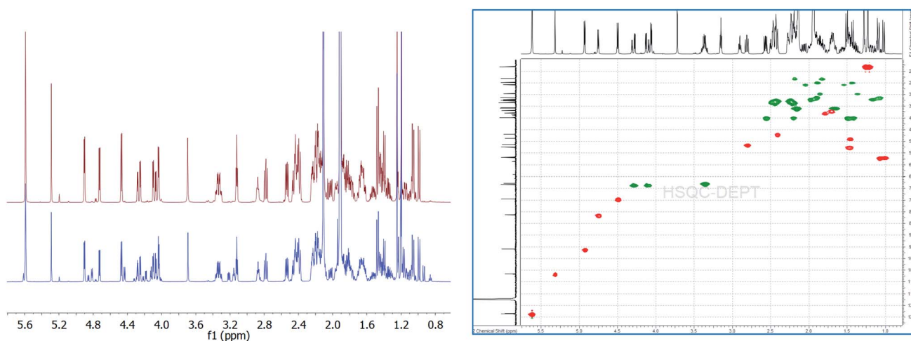
Fig. 1 Overlay of ^1\text{H}\{^{13}\text{C}\} NMR spectra of aldosterone 1 (S1: red; S2: blue) indicating the various diastereomers 2a , 2b , 3a , 3b along with the 2D-gHSQCAD spectrum (S1 material).
