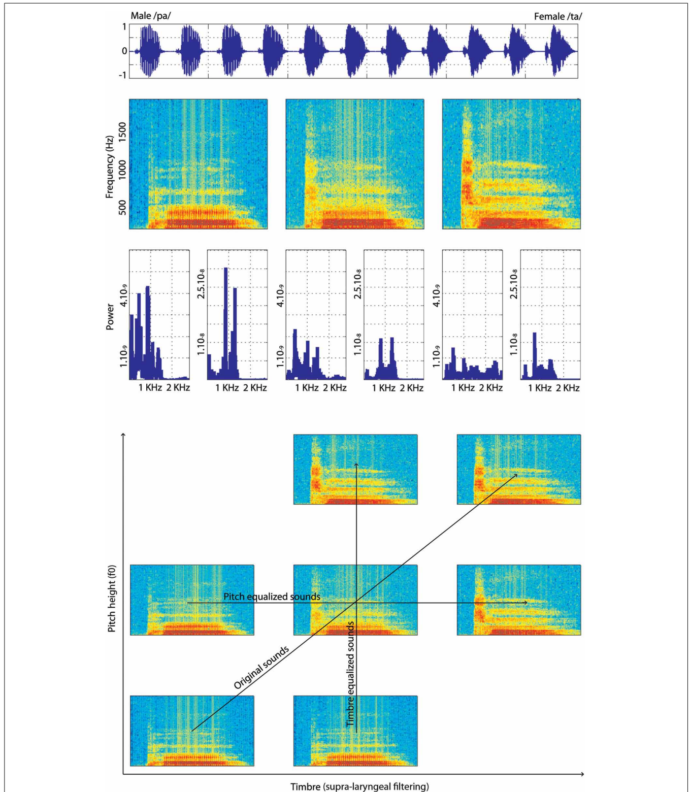
FIGURE 1 | Illustration of one continuum of male-/pa/ to female-/ta/. At the top is presented a male-/pa/ to female-/ta/ continuum in the time domain (waveforms). Below it, the time-frequency domain (spectrograms with hamming window, sampling at 22,040 Hz) of the 100% male-/pa/ stimulus, 50% male-/pa/, 50% female-/ta/ stimulus and 100% female-/ta/ stimulus from
