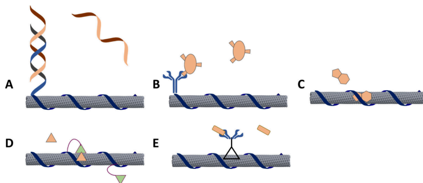
Figure 2. Common SWCNT functionalization methods with demonstrated functionality in vivo. In each panel, the gray tube represents a SWCNT transducer, the blue elements represent SWCNT functionalization methods, and the orange elements represent various analytes of interest. A) A method for complementary nucleic acid base pair detection. Dark blue ssDNA stabilizes SWCNTs in solution and light blue is complementary to the sequence of interest (orange). B) A method for protein antigen detection. Dark blue ssDNA stabilizes SWCNTs in solution and a light blue antibody is conjugated to it, which detects the analyte of interest (orange). C) A method of small molecule (orange) detection based on its interaction with dark blue ssDNA used to stabilize SWCNTs. The ssDNA may have some intrinsic or screened affinity for the analyte of interest. D) CoPhMoRe-based detection of a small molecule analyte (orange), wherein dark blue represents a screened polymer or ssDNA that has created binding pockets for the analyte. This may be enhanced by target templating, using conjugated target (purple). E) Integration of sp^3 carbon functionalization, termed organic color centers (OCCs) or quantum defects, which may impart selectivity for an analyte itself or, in this example, after conjugation with an antibody fragment.
