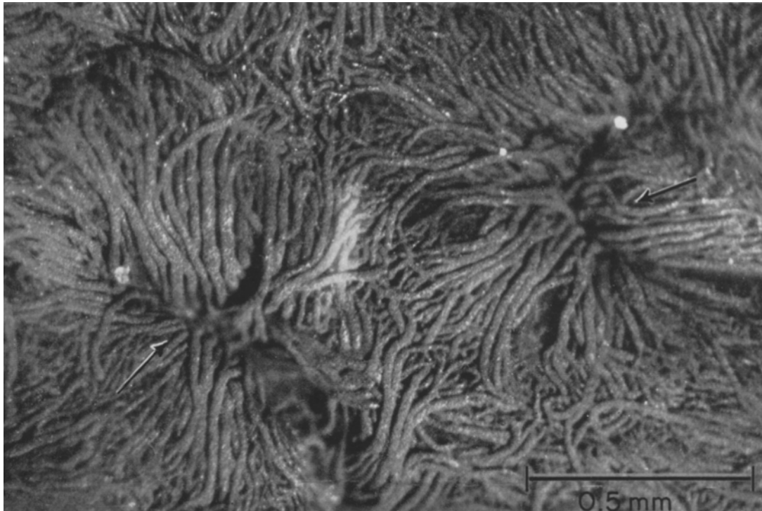
FIGURE 3. Photograph of the luminal surface of an India ink-injected bluefish gas-secreting complex showing the capillaries. Two areas in which the capillaries descend to their junctions with the underlying retia are indicated by arrows.
