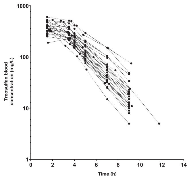
FIGURE 1 Full concentration–time profiles of treosulfan in 27 paediatric patients undergoing haematopoietic stem cell transplantation, receiving 14 g/m 2
