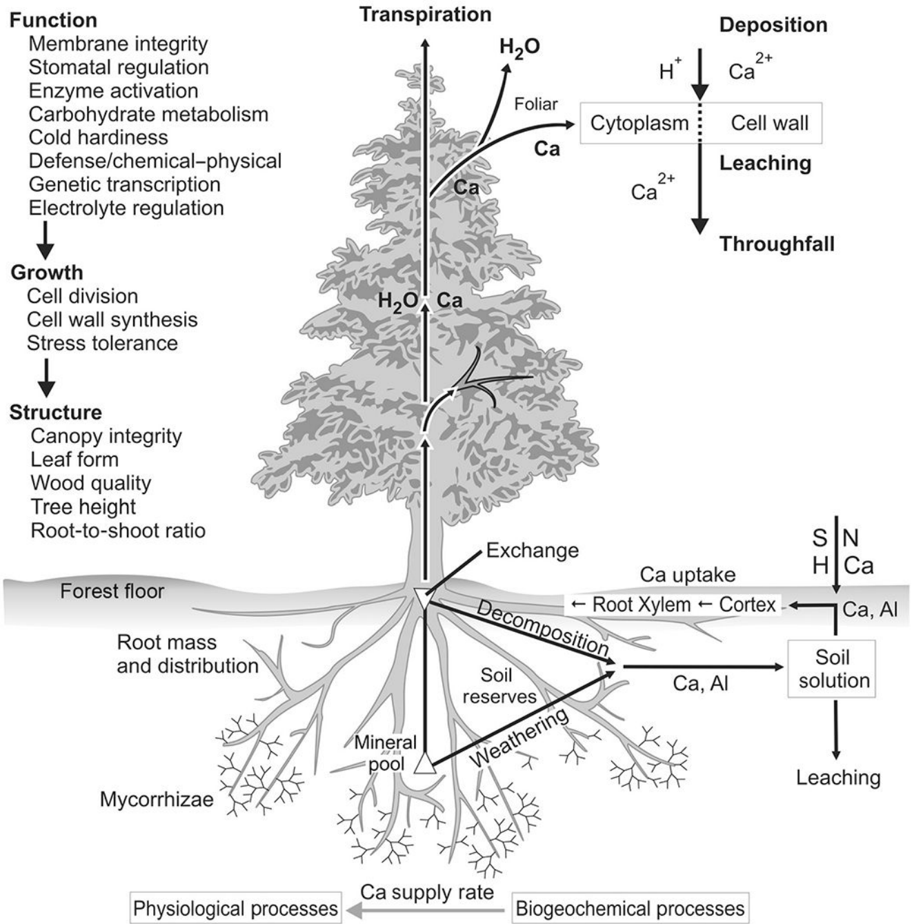
Fig. 2. Conceptual diagram of how nitrogen deposition alters calcium cycling and dependent tree and ecosystem structure and function. Modified from Fenn et al. 2006.
