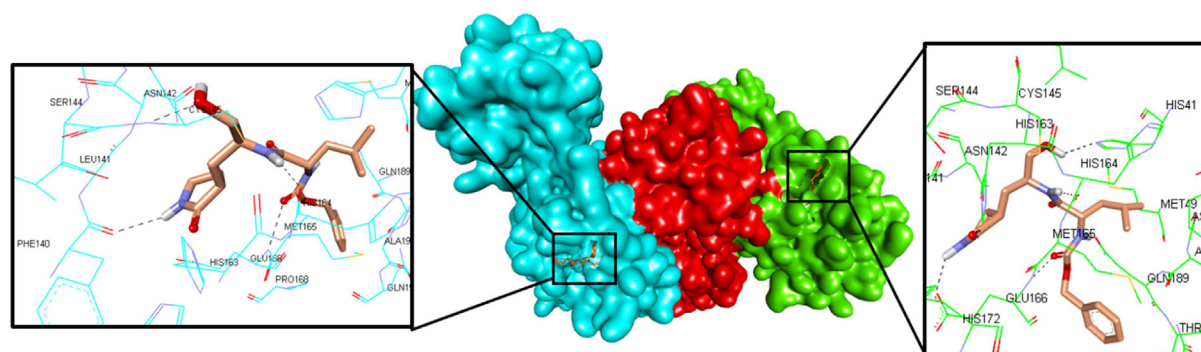
Fig. 6. The trimer structure of 3CLpro as indicated by blue (monomer A), red (monomer B), and green (monomer C) surface models. Inset is the ligand complex to the active site of the enzyme (presented by blue stick and green stick, for monomer A and monomer C, respectively), presented in a stick model (orange = C, white = H, blue = N and red = O). The H-bond is presented in black dot lines, respectively. (For interpretation of the references to colour in this figure legend, the reader is referred to the web version of this article.)
