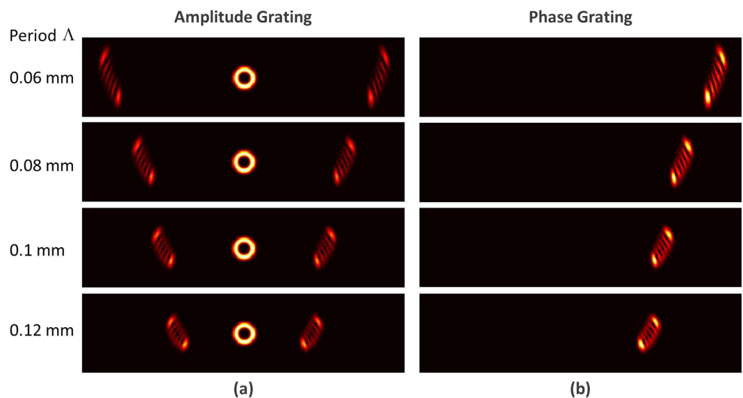
Figure 7. Simulation results of OAM states ( l = +5 ) measurement of vortex beams with annular gratings. (a) Amplitude grating with period \Lambda = 0.06 mm, 0.08 mm, 0.1 mm and 0.12 mm; (b) phase grating with period \Lambda = 0.06 mm, 0.08 mm, 0.1 mm and 0.12 mm.
