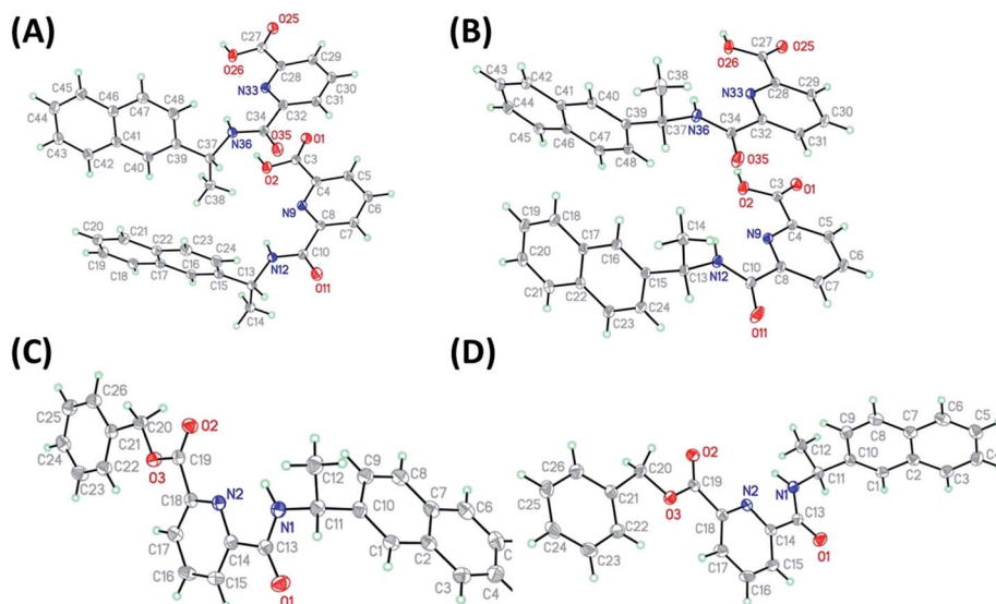
Fig. 2 Molecular structures of (A) \mathbf{1}(\mathbf{R}) and (B) \mathbf{1}(\mathbf{S}) showing both independent molecules in the asymmetric unit, (C) \mathbf{4}(\mathbf{R}) and (D) \mathbf{4}(\mathbf{S}) (thermal displacement 50%).
