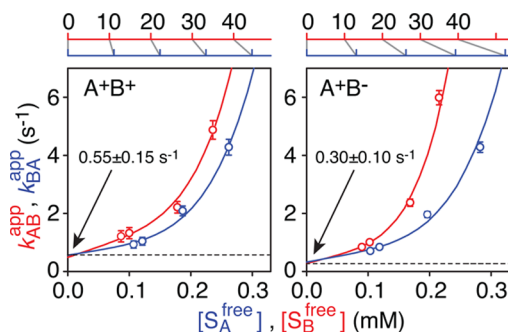
Figure 4. Dependence of apparent exchange rates on simultaneous variation of the concentrations of added \text{Na}^+ and free specific DNA sites. The data were obtained by successively diluting the original samples (cf. Figure 2) with 95% \text{H}_2\text{O}/5\% \text{D}_2\text{O} .
