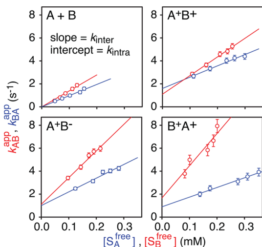
Figure 3. Dependence of k_{AB}^{\text{app}} and k_{BA}^{\text{app}} on the concentration of free DNA specific sites ( S_B^{\text{free}} and S_A^{\text{free}} , respectively). Experimental conditions as in Table 1 and Figure 2. For experiments with DNA- A^+B^+ , DNA- A^+B^- , and DNA- B^+A^+ , the ratio of DNA to protein was kept constant at 1.12:1 so that 80% of the DNA molecules have HoxD9 bound to one of the two specific sites and 20% have both specific sites occupied. The ratio of DNA-A and DNA-B to HoxD9 was kept constant at 1:1:1.
