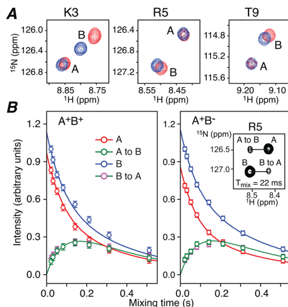
Figure 2. TROSY-based ^{15}\text{N}_z -exchange spectroscopy. (A) Examples of cross-peaks with different ^{15}\text{N}/^1\text{H}_\text{N} chemical shifts when bound to the A and B sites of DNA- \text{A}^+\text{B}^+ (blue) and DNA- \text{A}^+\text{B}^- (red). (B) Dependence of the intensities of auto and exchange cross-peaks on mixing time ( T_{\text{mix}} ) in the TROSY-based ^{15}\text{N}_z -exchange spectra (open circles) together with the best-fit curves (solid lines) obtained using a simple model for a phenomenological pseudo-first-order exchange reaction (see SI). The experimental intensities, for display purposes (see SI), represent the averages for Lys3, Arg5, and Thr9. The inset in the right panel shows the auto and exchange cross-peaks for Arg5 at T_{\text{mix}} = 22 ms. Experiments were performed at 600 MHz and 25 °C on samples of 0.45 mM uniformly ^2\text{H}/^{15}\text{N} -labeled HoxD9 and 0.40 mM DNA duplex (DNA- \text{A}^+\text{B}^+ or DNA- \text{A}^+\text{B}^- ) at natural isotopic abundance in buffer containing 20 mM HEPES/5 mM \text{Na}^+ -HEPES, pH 7.0, 30 mM NaCl, and 95% \text{H}_2\text{O}/5\% \text{D}_2\text{O} (see SI).
