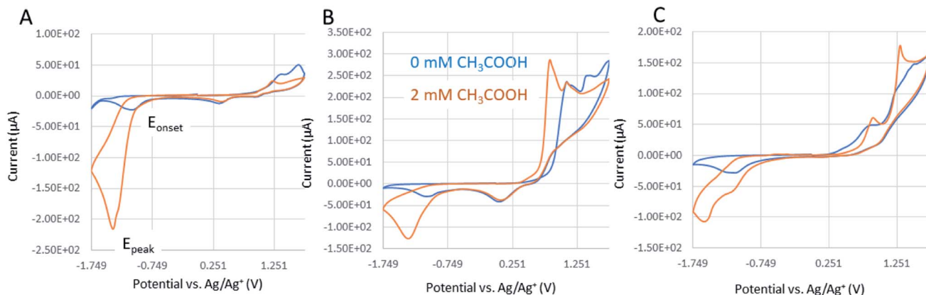
Fig. 9 Cyclic voltammograms of 1 mM catalyst in electrolyte for \text{Co(II)Cl}_2 reference (A); [\text{Co}_6\text{Na}(\text{NCMe})_6(\mu\text{-O})(p\text{-tert-butylcalix[6]areneH})_2\text{Br}] \cdot 7\text{MeCN} (6·7MeCN) (B); and [\text{Co}_4\text{Na}(\text{NCMe})_4(\mu\text{-O})(p\text{-tert-butylcalix[8]arene})(p\text{-tert-butylcalix[8]areneH}_5)\text{Br}] \cdot 13\text{MeCN} (7·13MeCN) (C) in dry 0.1 M \text{TEABF}_4 in MeCN at a potential scan rate of 0.1 \text{ V s}^{-1} recorded in the absence (blue) and presence of the acetic acid substrate (orange; 2 mM equivalent with respect to catalyst concentration).
