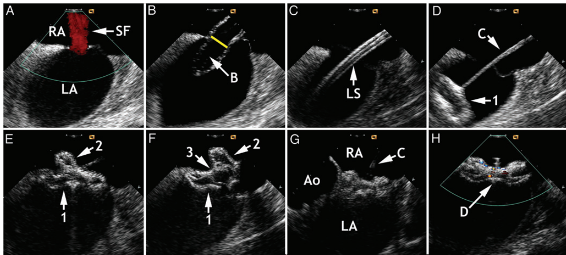
Figure 3 Atrial septal defect device closure: (A) longitudinal view showing left-to-right shunt; (B) balloon sizing; (C) long sheath with wire inside; (D) opened left-sided disc in the left atrium; (E) release of right-sided disc in the right atrium; (F) 'wiggle manoeuvre'; (G) short-axis view and (H) longitudinal view with the device in place. 1, left-sided disc; 2, right-sided disc; 3, stent; Ao, aorta; ASD, secundum type atrial septal defect; B, balloon; C, cable; D, device; LA, left atrium; LS, long sheath; RA, right atrium; SF, shunt flow.
