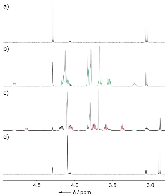
Figure 4. Partial ^1\text{H} NMR spectrum (500 MHz, \text{CD}_3\text{CN} , 298 K) of a) E - 2b , b) 1 : 1 mixture of E - 2b and 1 (5 mM; the signals of the E complex are highlighted in green), c) equilibrated 1 : 1 mixture of 1 and Z - 2b , obtained upon exhaustive irradiation of E - 2b ( \lambda_{\text{irr}} = 365 nm, 30 min; 5 mM; the signals of the Z complex are highlighted in red), and d) Z - 2b , obtained upon exhaustive irradiation of E - 2b at 365 nm.
