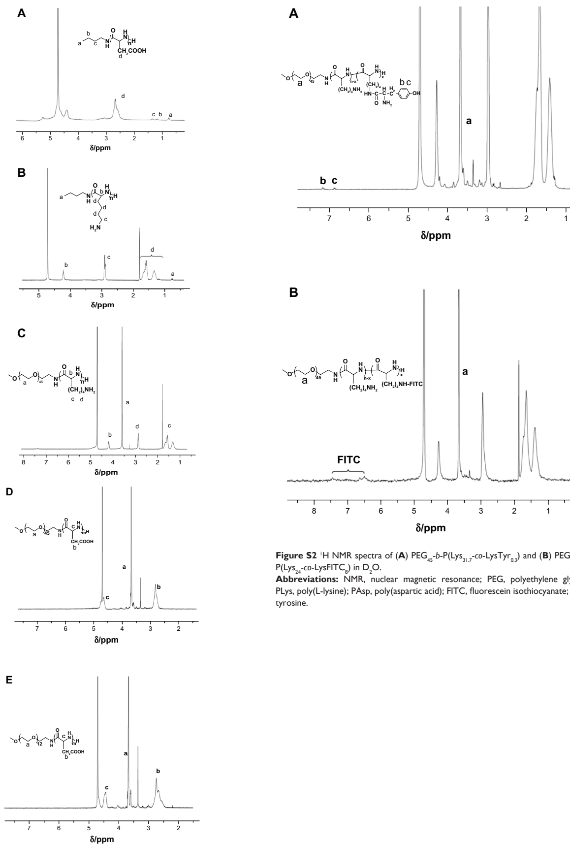
Figure S1 ^1\text{H} NMR spectra of (A) PAsp 32 , (B) PLys 18 , (C) PEG 45 -b-PLys 32 , (D) PEG 45 -b-PAsp 36 , and (E) PEG 12 -b-PAsp 16 in D 2 O.
